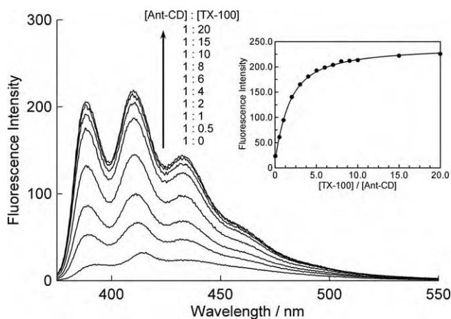
Fig. 2. Fluorescence spectra of Ant-CD and its TX-100 complex in water at 25 °C. Excitation wavelength: 363 nm. [Ant-CD] = 5 μM. Molar ratios for TX-100 are listed in columns. Inset: dependence of fluorescence intensity at 410 nm on the concentration of TX-100, and its theoretical curve for formation of stoichiometric 1:1 complex.
