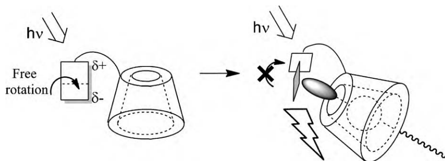
Fig. 1. Fluorescence switching by TICT-inhibiting process outside CD cavity in the presence of target material.
