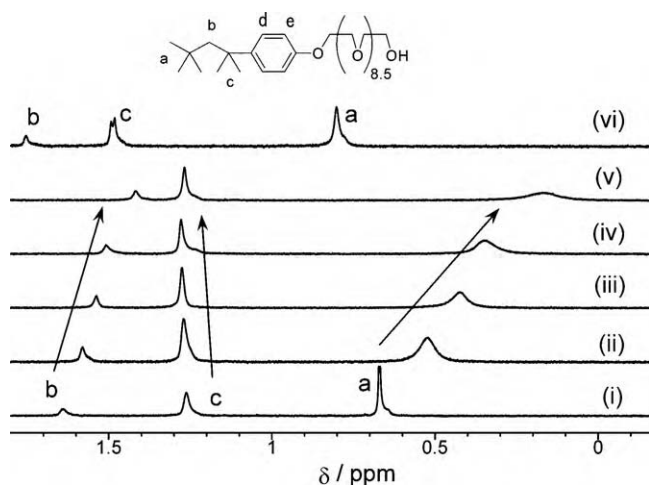
Fig. 3. ^1\text{H} NMR spectra of TX-100 before and after inclusion into Ant-CD. (i) 0 mM, (ii) 0.3 mM, (iii) 0.5 mM, (iv) 0.7 mM, (v) 1.2 mM of Ant-CD with 1 mM of TritonX-100, and (vi) 1 mM of native \beta -CD with 0.5 mM of TX-100 in \text{D}_2\text{O} at 30^\circ\text{C} .
